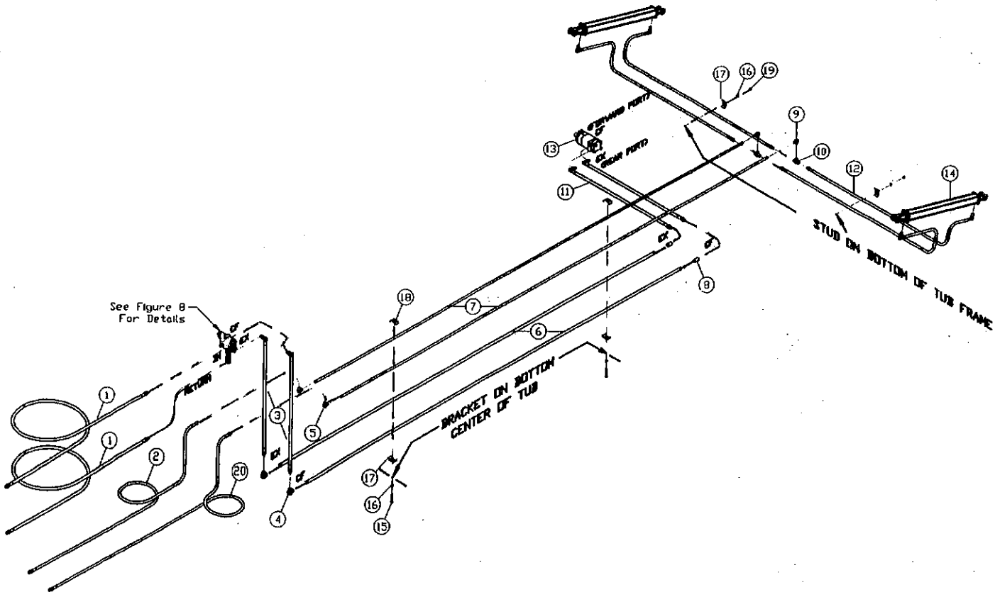
FIGURE 9 HYDRAULICS ASSEMBLY
