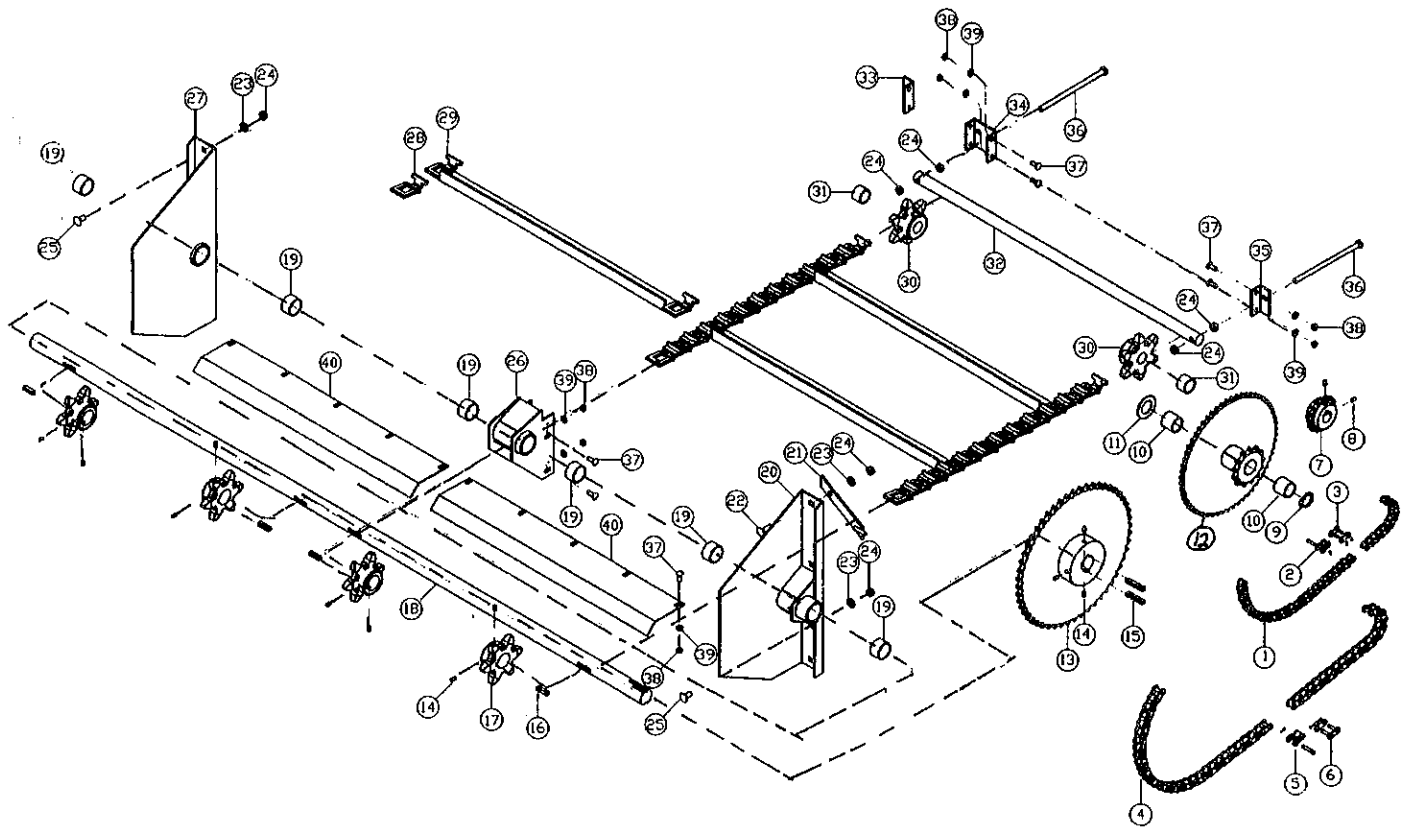
FIGURE 6 APRON CHAIN & DRIVE ASSEMBLIES
