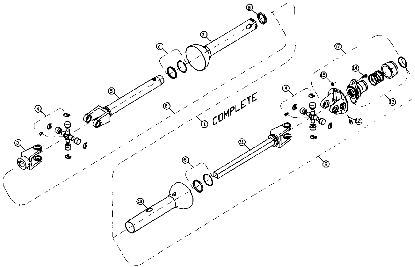
FIGURE 12 PTO ASSEMBLIES
